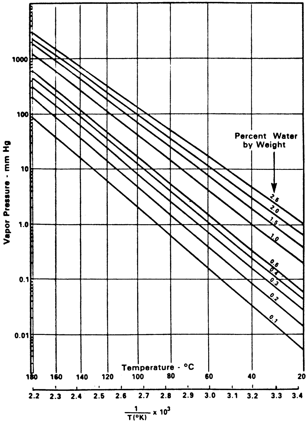
Figure A.2—Equilibrium chart relating water vapor pressure over oil to water concentration in kraft paper vs. temperature
