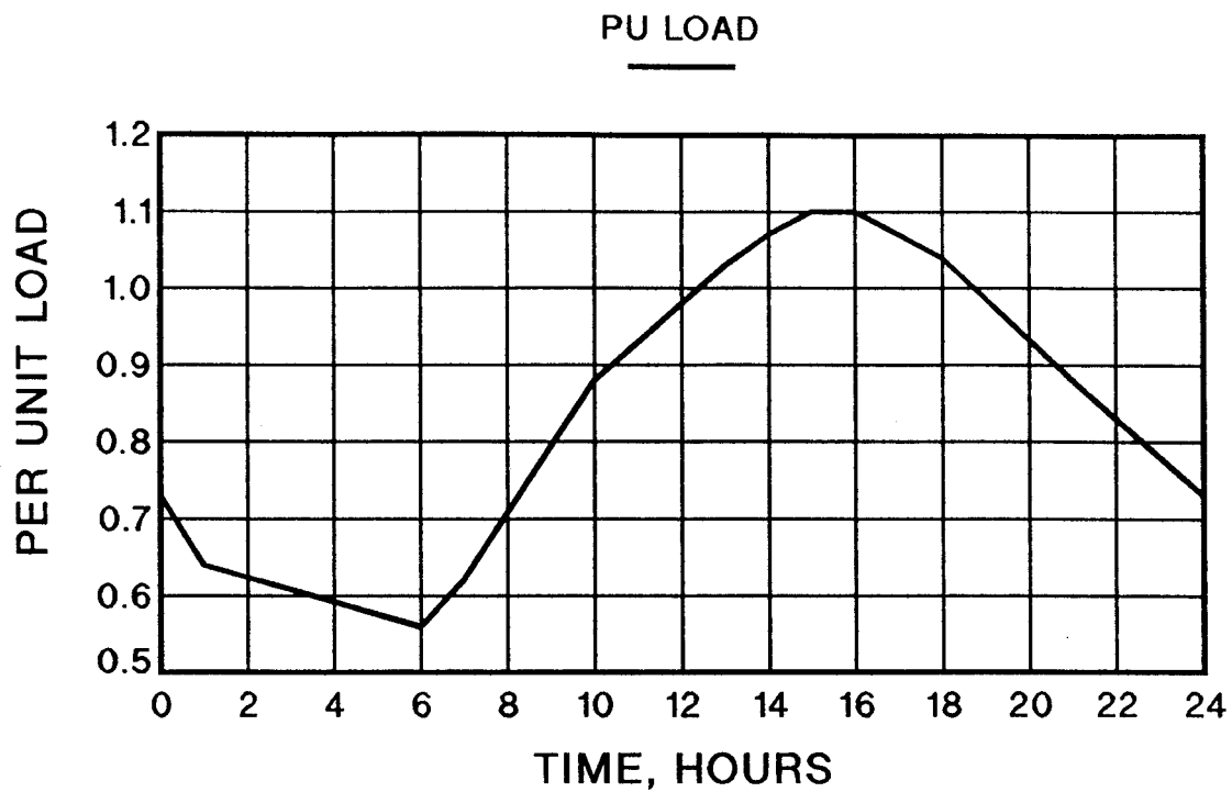
Figure G.1—Example load cycle
