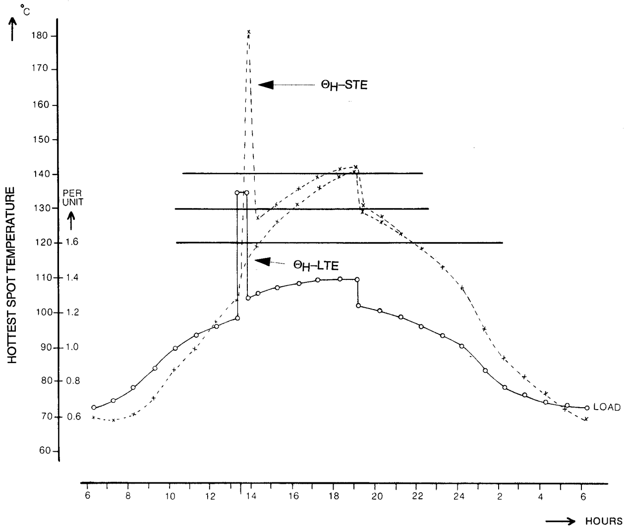
Figure C.2—Hottest-spot temperature profile for long time and short time emergency loadings
