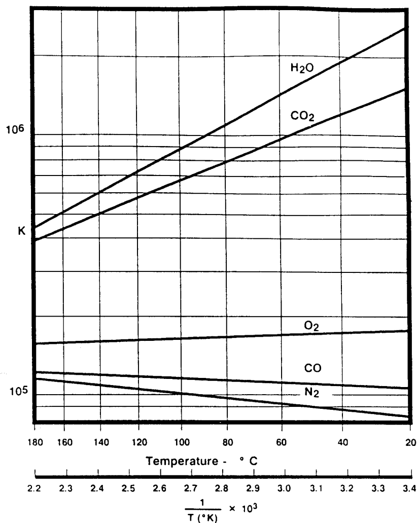
Figure A.3—Henry's Law constants (ppm vol/atm) for common gases in mineral oil
