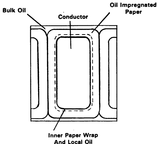
Figure A.1—Insulated winding conductor subsystem within a transformer
